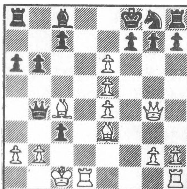
243 After 17...Qb4
